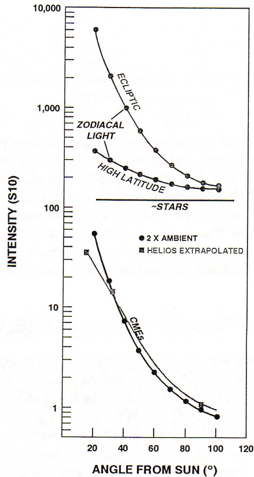
Figure 1. The brightness of various signals observed by the imager versus elongation at 1 AU.
