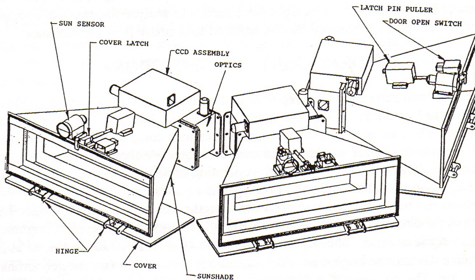
Figure 3. Layout of the proposed SMEI.
